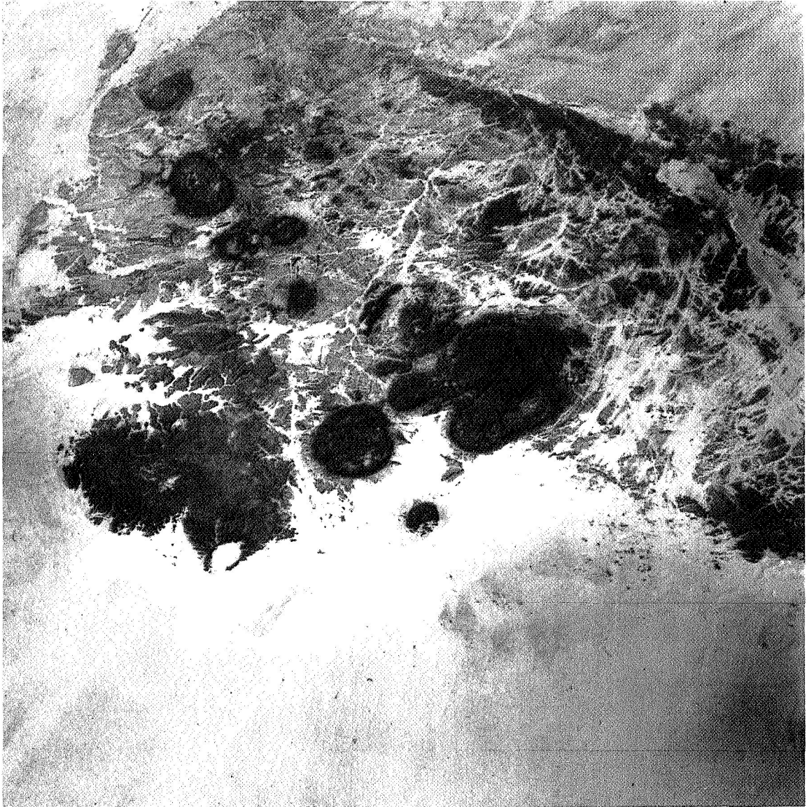
Figure 27. Gemini 6-A photograph S-65-63158. View to southwest over Niger. Desert with sif dunes in foreground is the Tenere; Air Mountains at center (about 19^{\circ}\text{N} , 8^{\circ}\text{E} ). Dark masses are peralkaline granite intrusions; largest (at center) is Mont Tamgak, roughly 30 miles (48 km) wide, intruding metamorphic rocks. Plateau of Irhaouriten, underlain by sandstone, in upper right. Linear features north of Mont Tamgak appear to be wind-eroded ridges and sand streamers; note continuity with sif dunes in foreground. Steep-cliffs around intrusions are suggestive of examples of wind erosion pictured by Holmes (1965).
